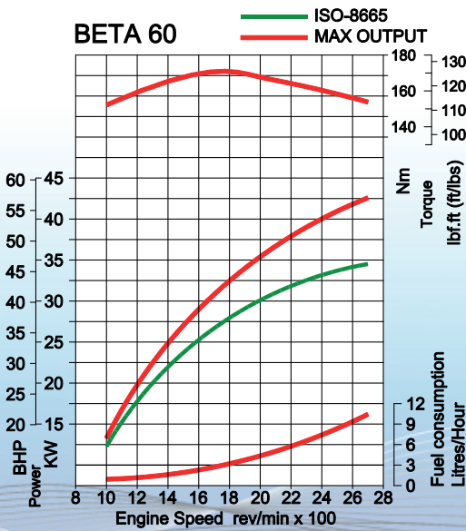
Based on theoretical propeller loading - matched at full speed
